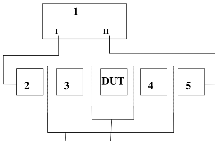
Figure II (a) - VECTORIAL METHOD OF RF INSERTION LOSS MEASUREMENT OF CABLE ASSEMBLIES
