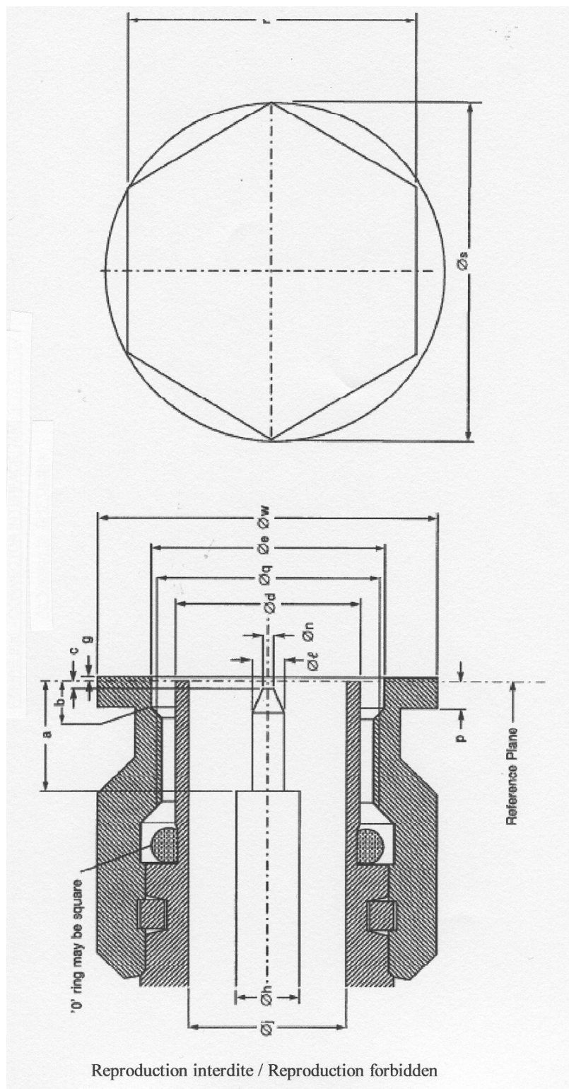
FIGURE 2(a) CONNECTOR INTERFACE MALE CONTACT AIR VERSION (Frequency range DC/18 GHz)
