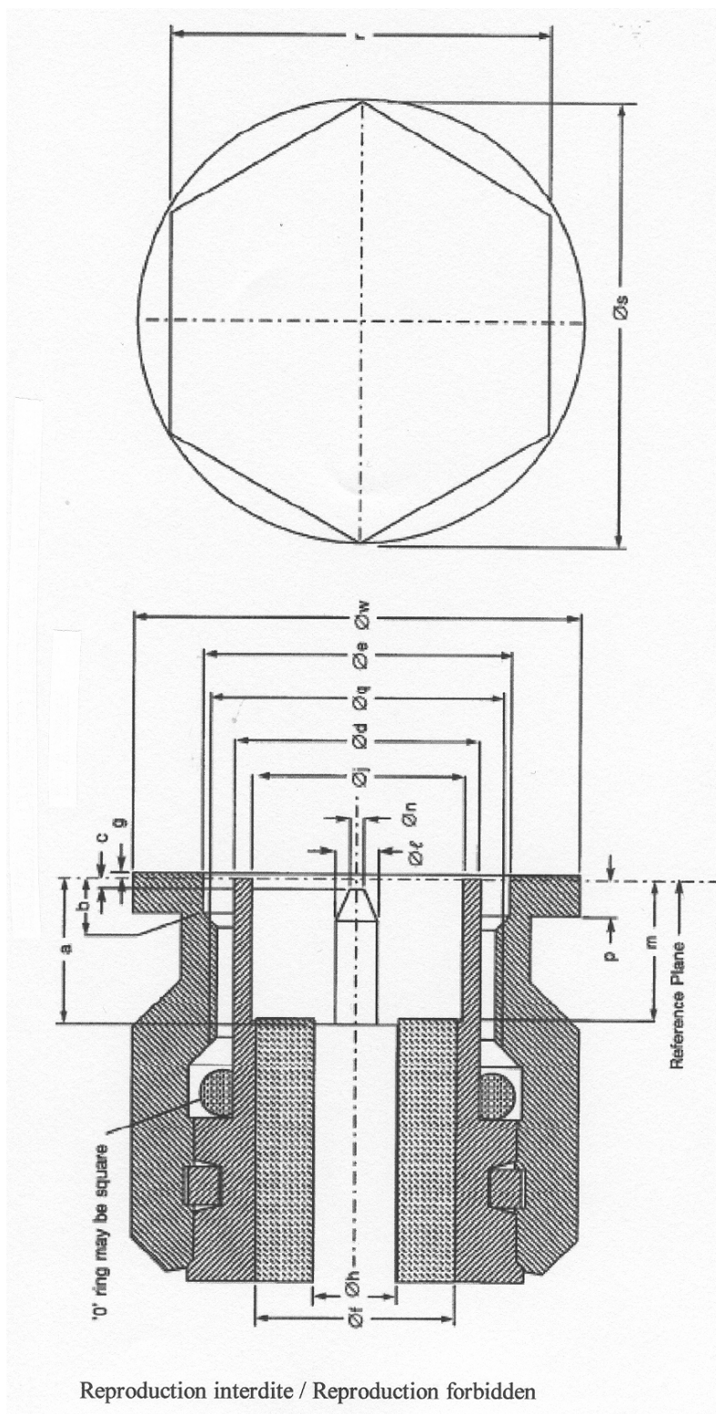
FIGURE 2(a) – CONNECTOR INTERFACE, MALE CONTACT (CONTINUED) PTFE VERSION (Frequency range DC/18 GHz)
