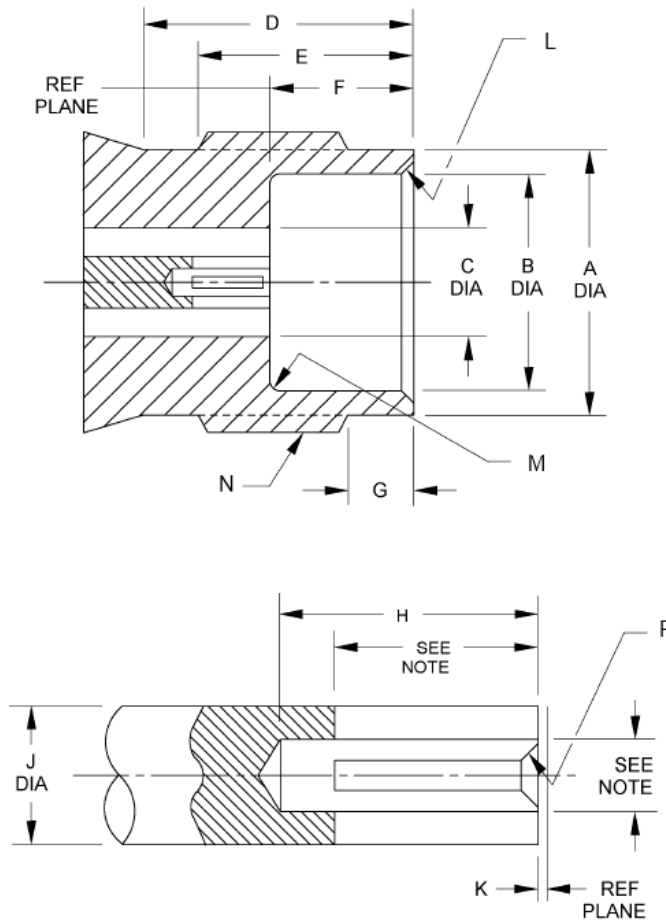
FIGURE 3 (a) – STANDARD TEST CONNECTOR INTERFACE, FEMALE CONTACT
