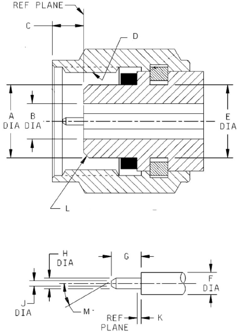
FIGURE 2(a) – CONNECTOR INTERFACE MALE CONTACT
