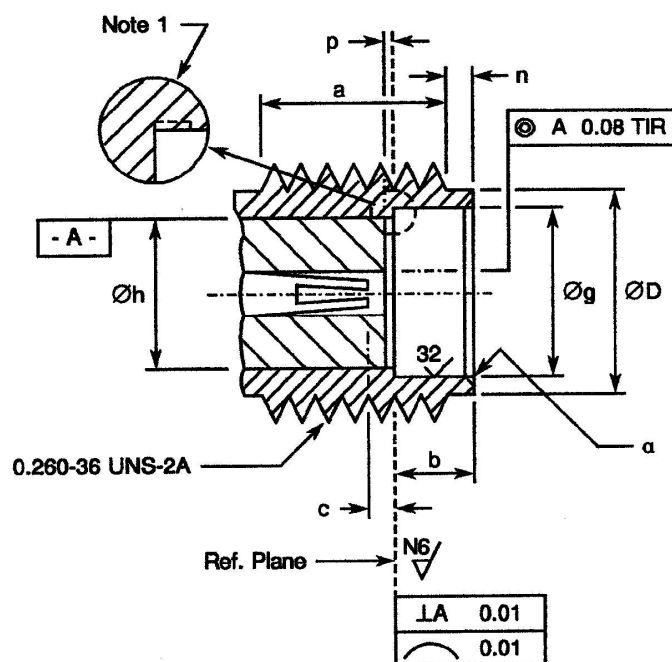
FIGURE 3 – STANDARD TEST CONNECTOR INTERFACE – FEMALE CONTACT
