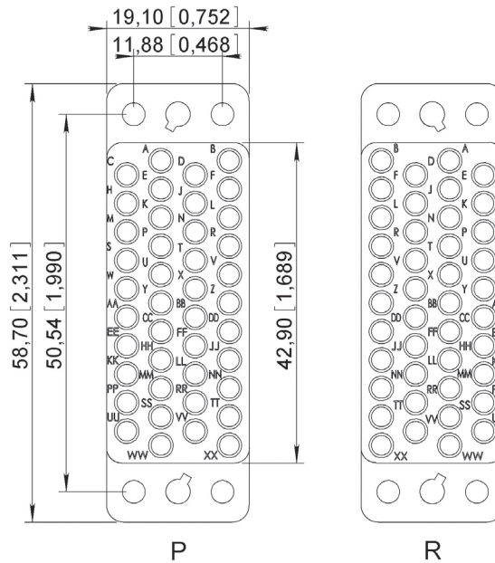
42 contacts
