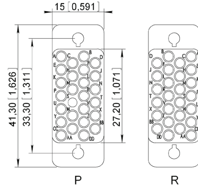
26 contacts
