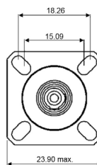
LxC-R® Square Flange Receptacle
