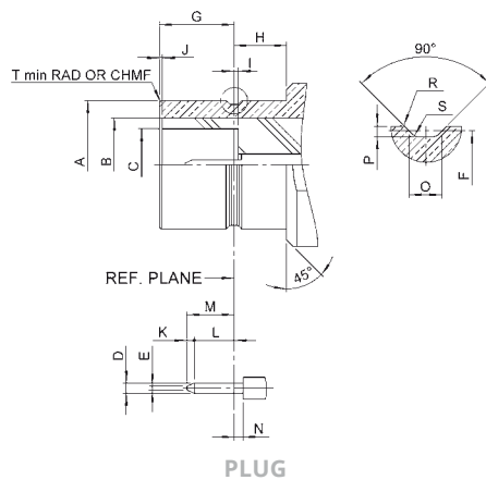
PLUG
