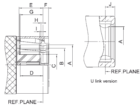
JACK
